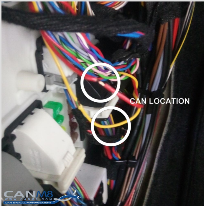
Yellow & Red CAN wires
