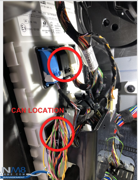
BDC Showing CON 8 Harness
